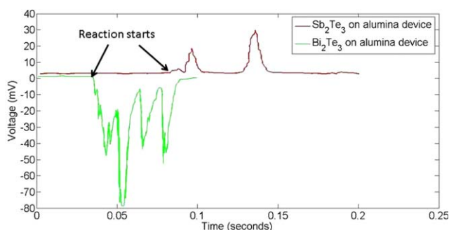
Figure 8. Oscillatory voltage output from thermopower waves devices using Sb 2 Te 3 on alumina and using Bi 2 Te 3 on alumina.
